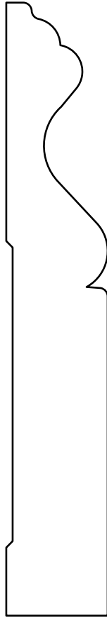
HBS219 3/4" x 4-1/2"
